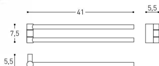
INCH 16.1x2.2x2.9
