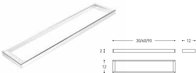
INCH 11.8/23.6/35.4x4.7x0.8
