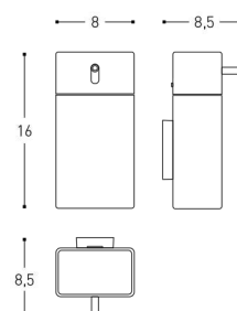
INCH 3.1x3.3x6.3
