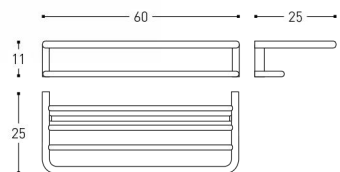
INCH 23.6x9.8x4.3
