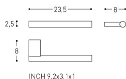
INCH 9.2x3.1x1
